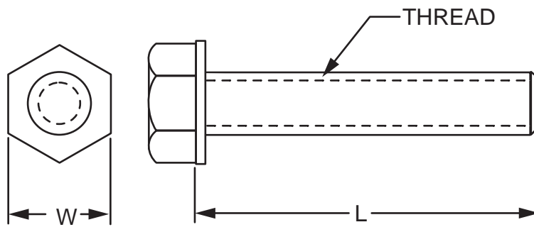
ORDERING TABLE
